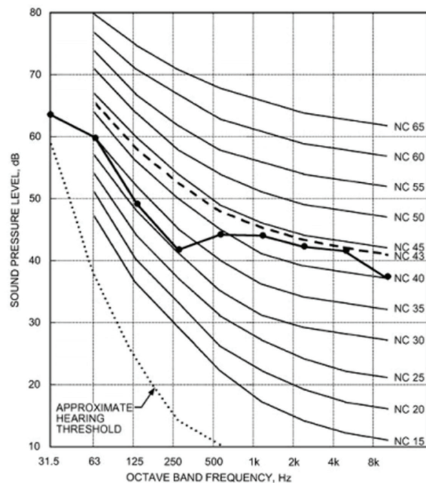
Figure 1 NC (Noise Criteria) Curves and Sample Spectrum (Curve with Symbols) 2017 ASHRAE Fundamentals Handbook Chapter 8
