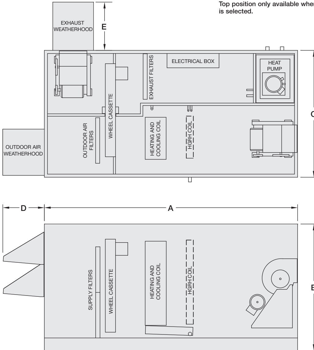
Drawings show optional hot gas reheat coil.
