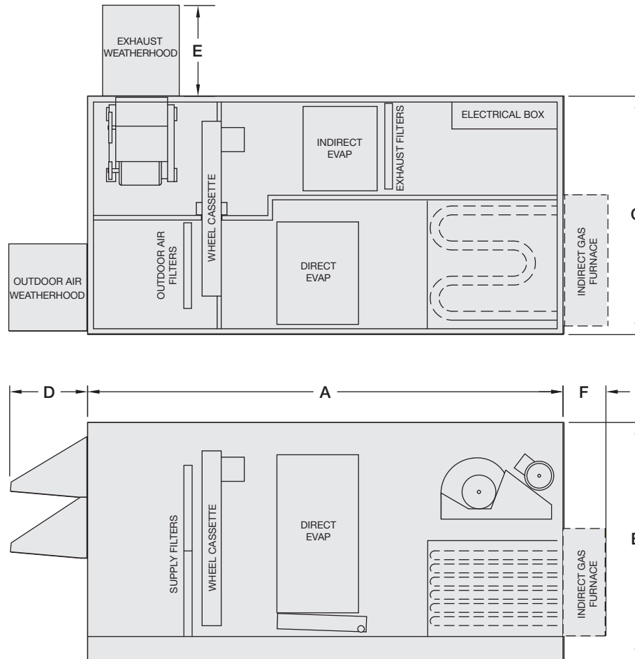
Drawings show optional indirect gas furnace. Electric heat is also available. Only one can be selected.
