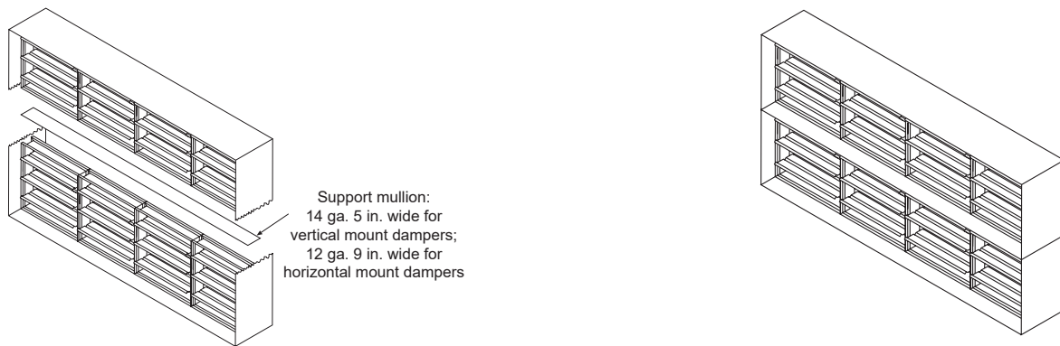
Figure 2: Two individually sleeved units with no mullions
