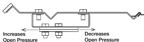
Figure 9: Counterweight adjustment for start open pressure. Blade is shown in full close position.
