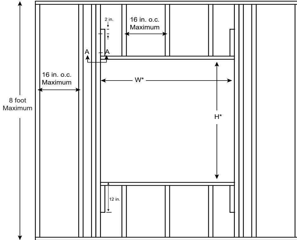
Figure 1: Framing Detail
