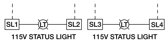
Example of two 115 VAC Status Lights
