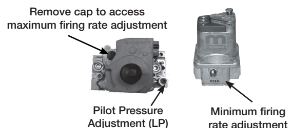
Fig. 4 Separate Regulator & Modulating Valves
