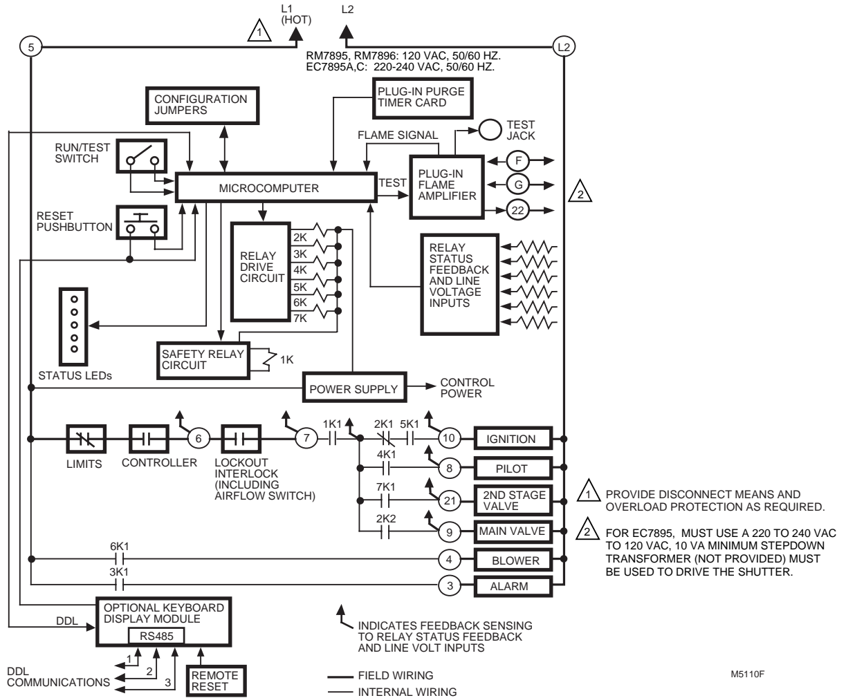
Fig. 1. Internal block diagram of RM7895A,B,C,D/EC7895A,C; RM7896A,B,C,D (see Fig. 2 and 3 for detailed wiring instructions).
