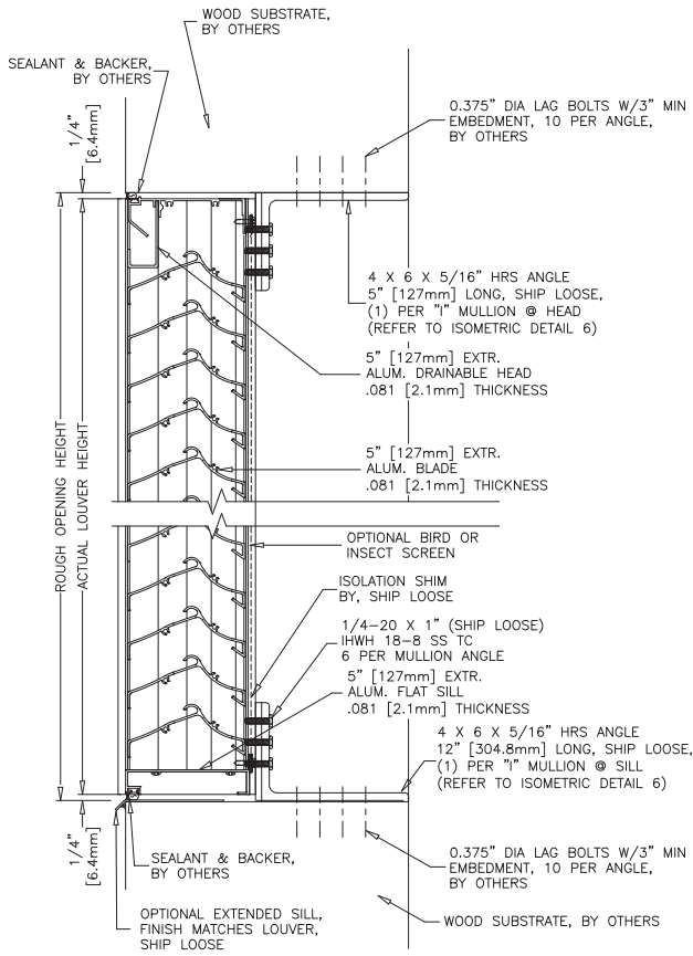
B SILL DETAIL MULTI SECTION WOOD
