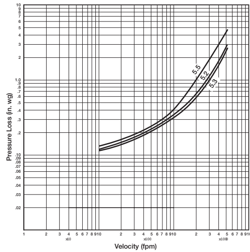
12 in. x 12 in. (305mm x 305mm) Damper
