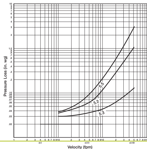
36 in. x 36 in. (914mm x 914mm) Damper
