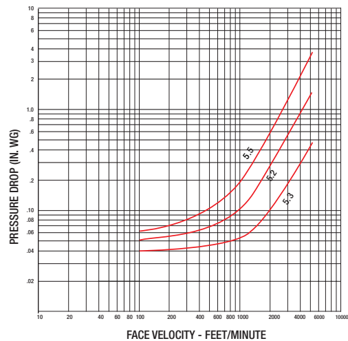
24 in. x 24 in. (610mm x 610mm) Damper
