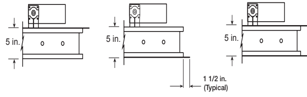
Single Flange
