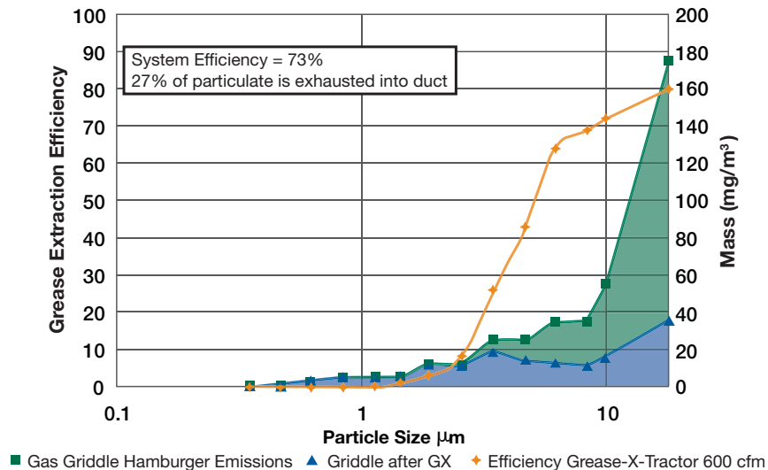
Mass & Grease Extraction Efficiency vs. Particle Size for Grease-X-Tractor™ Over Griddle with Hamburger
