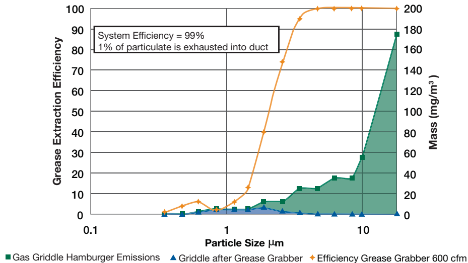
Mass & Grease Extraction Efficiency vs. Particle Size for Grease Grabber™ Over Griddle with Hamburger
