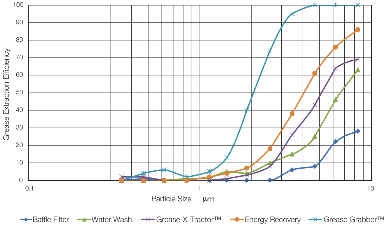
Grease Extraction Efficiency vs. Particle Size 600 CFM
