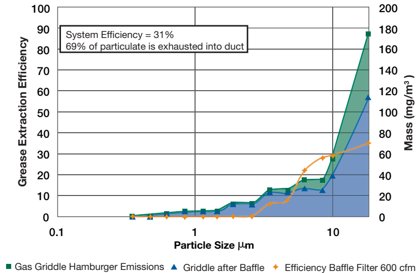
Mass & Grease Extraction Efficiency vs. Particle Size for Baffle Over Griddle with Hamburger
